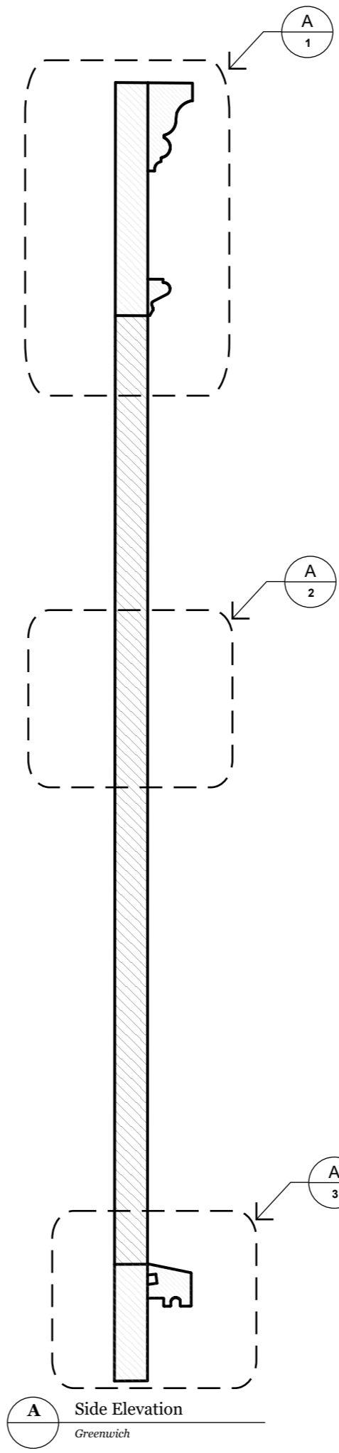
A 1" x 7 - 1/4" Top W/ Imperial Rake Crown & Base Cap Greenwich
