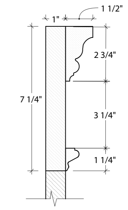
A 1" x 7 - 1/4" Top W/ Imperial Rake Crown & Base Cap Greenwich
