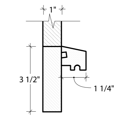
A 1" x 3 - 1/2" Skirt Greenwich
